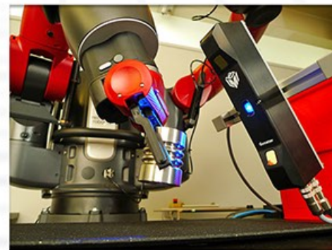
Parts inspection with LMI and Baxter Robot
